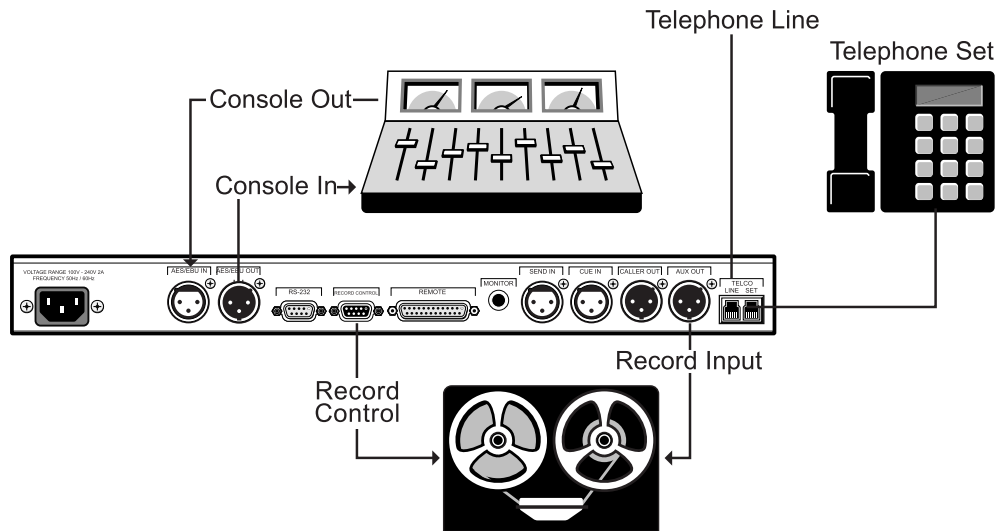
TYPICAL DH30 DIGITAL INSTALLATION
