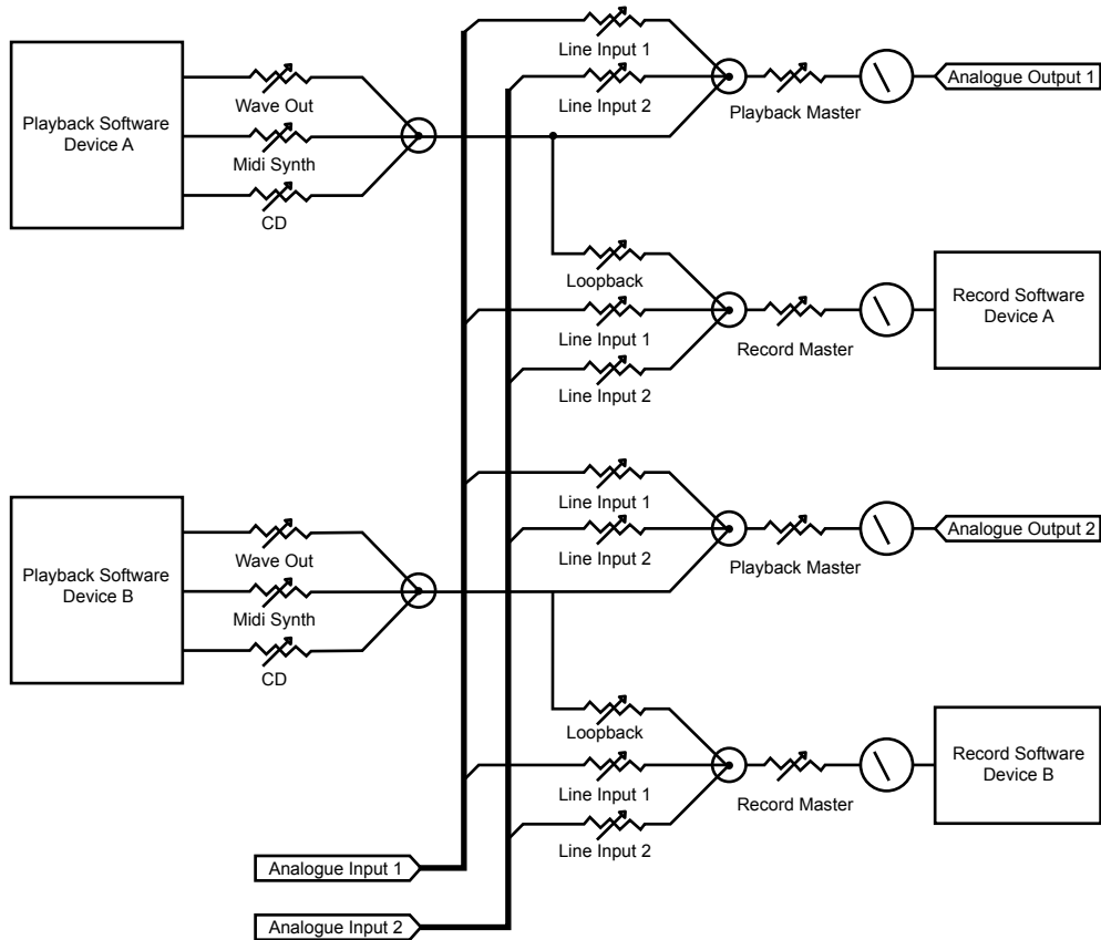
Fig 1-5: Auricon 4.4 Topology
