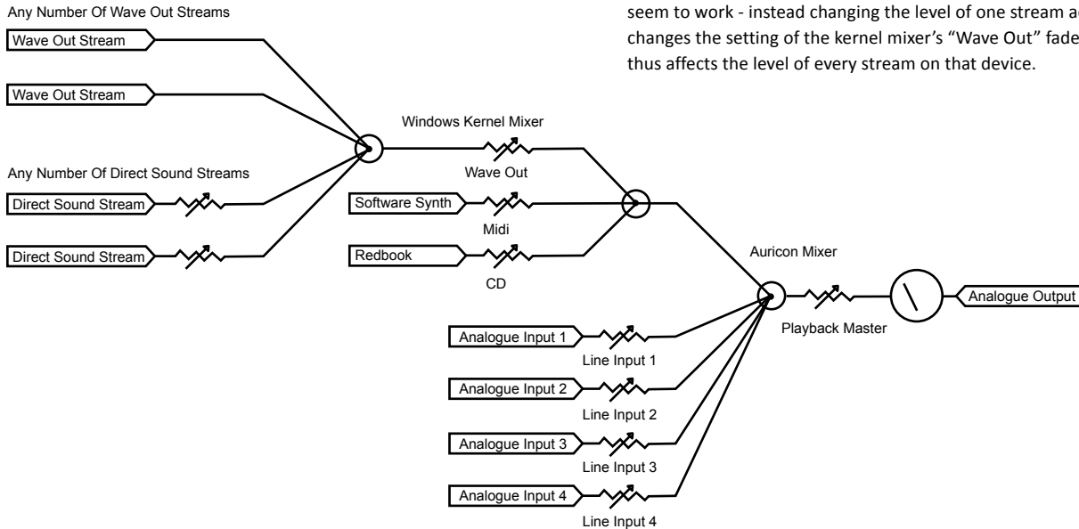
Fig 1-6: Output Mixing
